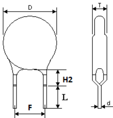
E→一字形腳(Vertical crimped)
